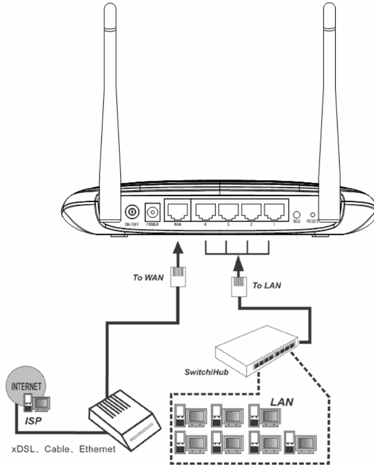
Figure 2-1 Hardware Installation of the TL-WR841ND 300Mbps Wireless N Router
